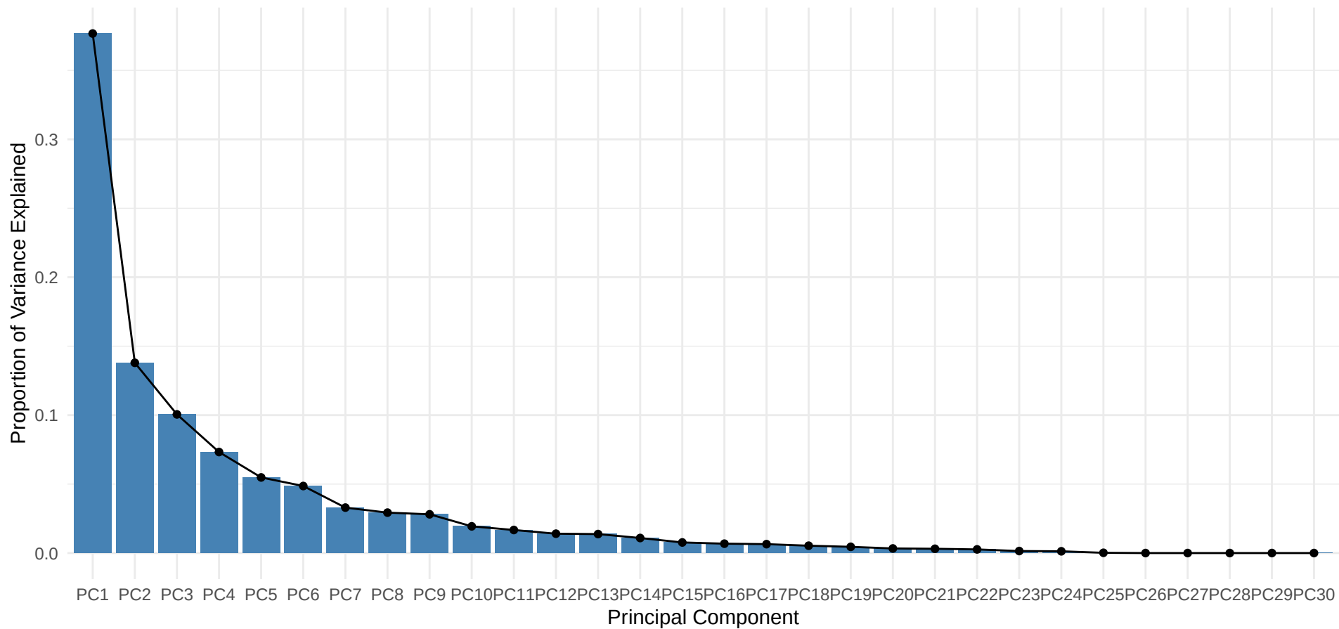
Scree Plot of PCA for Participant 7
